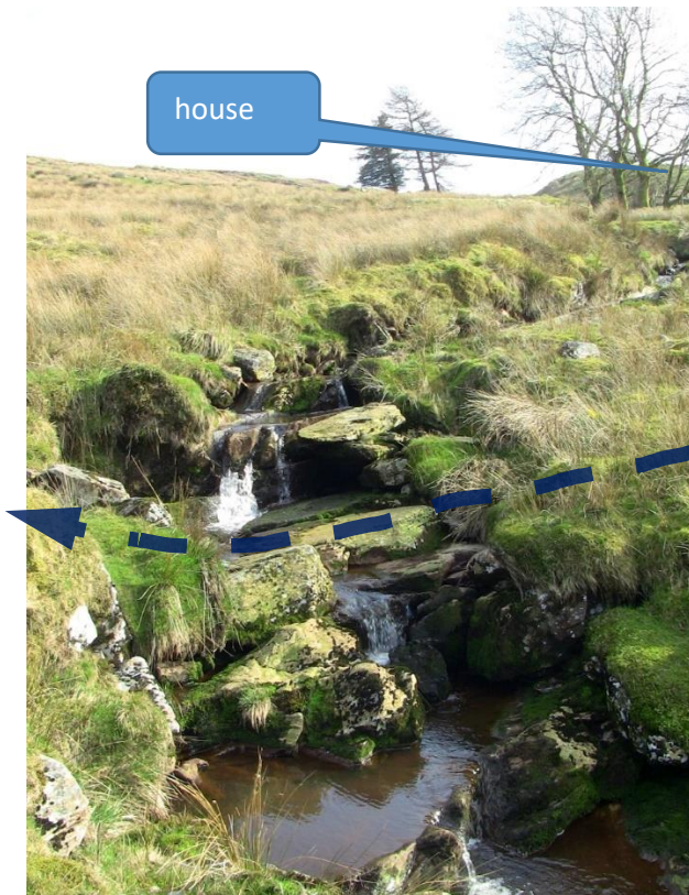
Figure 9. Second crossing point. The pipe will have an air-relief valve near each crossing point.
